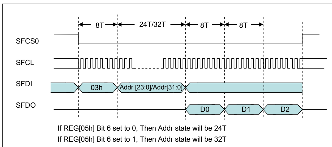
Figure 6-37 : 4-BUS (Normal) Read
