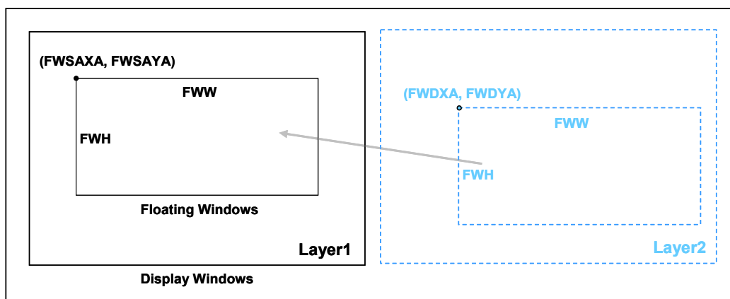
Figure 5-9 : Floating Windows
