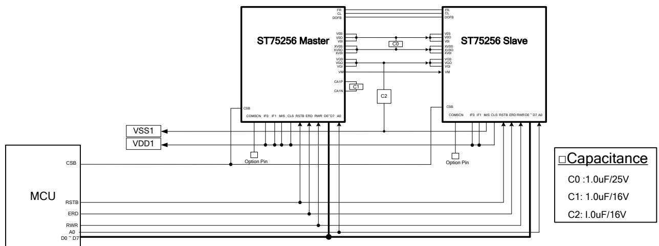
(2) Application Circuit of Internal Power Supply (8080 interface)
