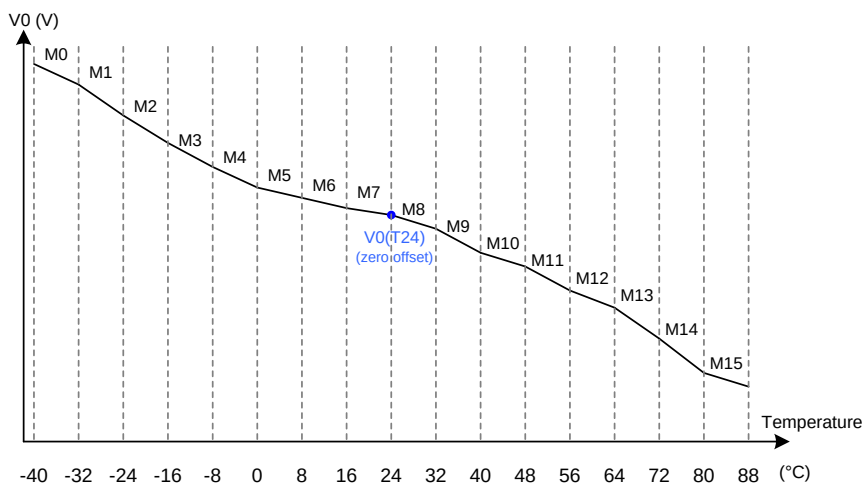
Figure 36 Temperature Gradient Compensation
