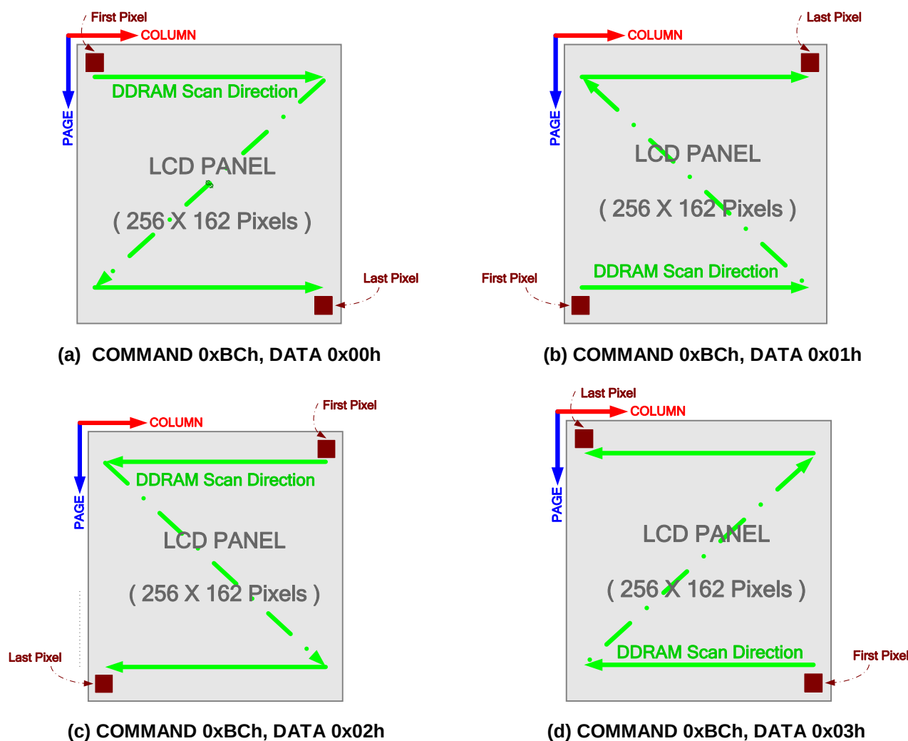
Figure 38 Different RAM accessing setup under COMMAND 0xBCh
