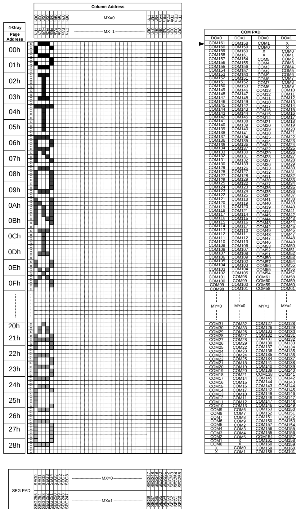
Figure 27 DDRAM Display Direction (4-Level Gray Scale Mode; COMSCN=1)
