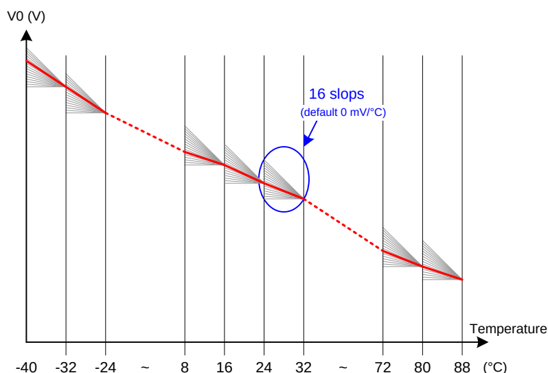
Figure 35 Temperature Compensation Coefficient Selection
